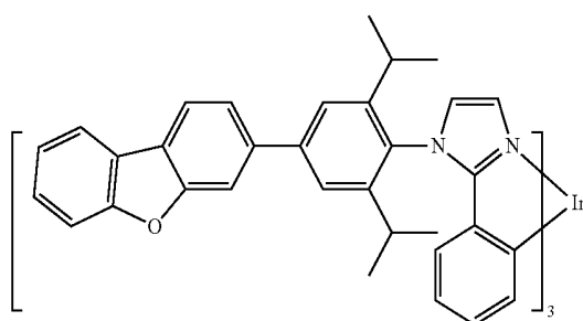
Compound 36
