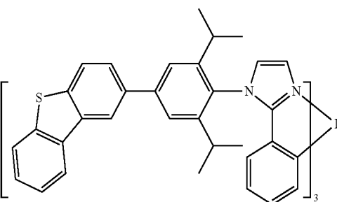
Compound 32
