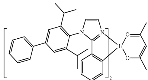
Compound 49
