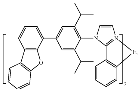
Compound 37
