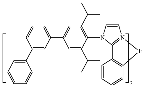
Compound 30
