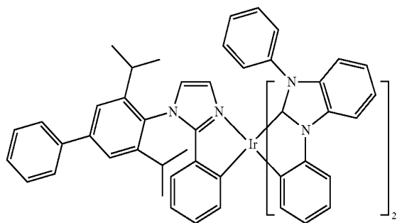
Compound 68
