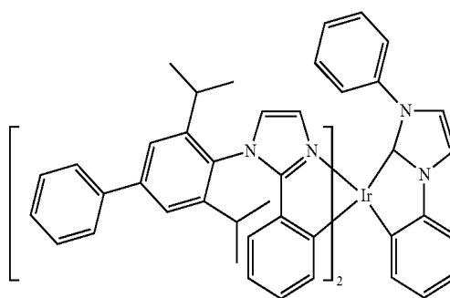
Compound 55
