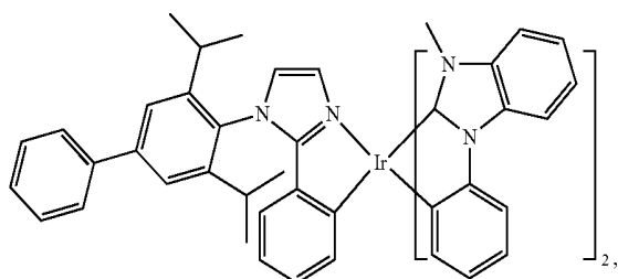
Compound 66
