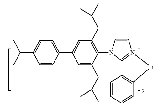
Compound 12
