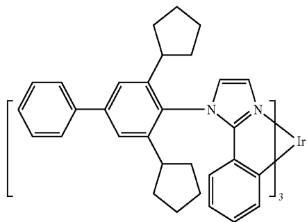
Compound 8
