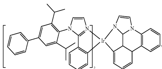
Compound 57
