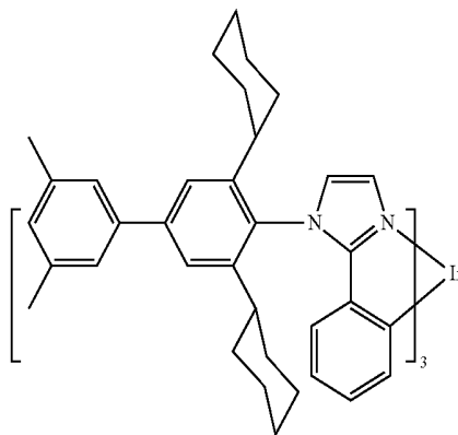
Compound 9
