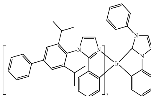
Compound 55
