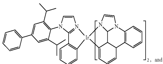
Compound 68
