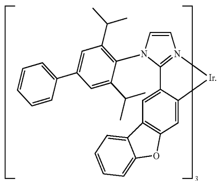
Compound 7
