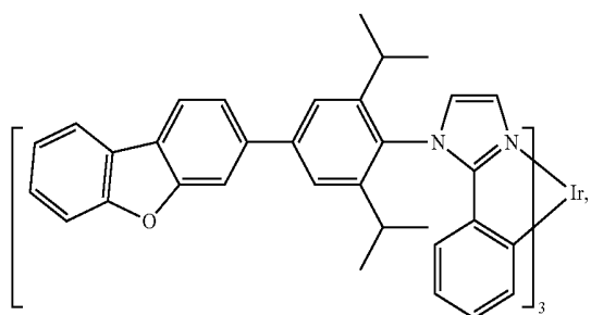
Compound 36
