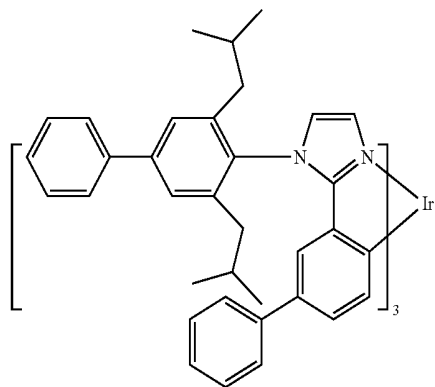
Compound 17
