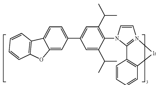
Compound 37
