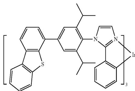
Compound 35
