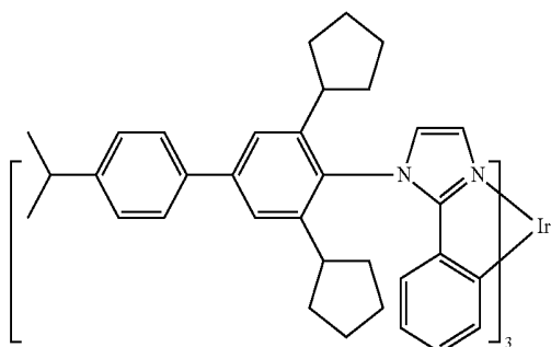
Compound 10
