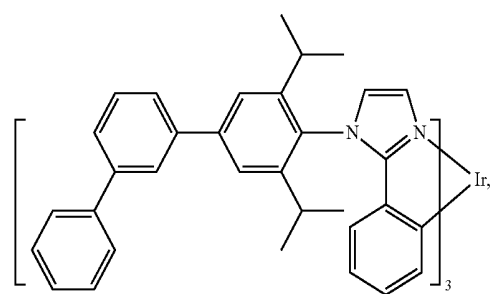
Compound 30
