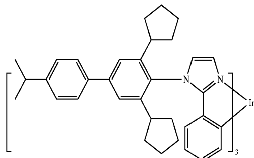
Compound 11
