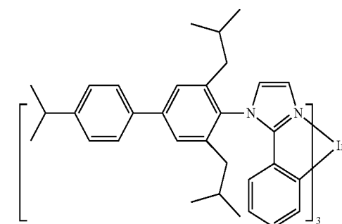
Compound 13
