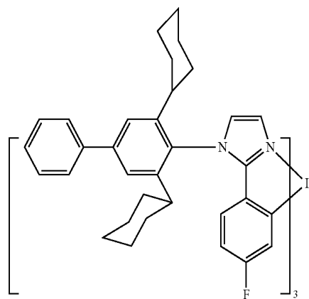
Compound 28
