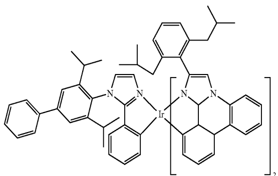
Compound 69
