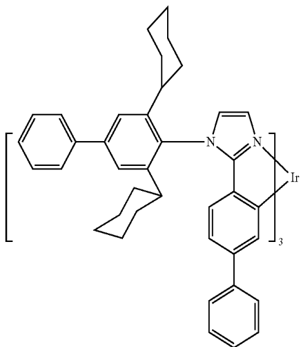
Compound 23
