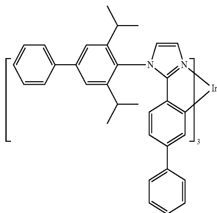
Compound 24
