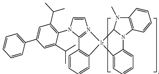
Compound 66
