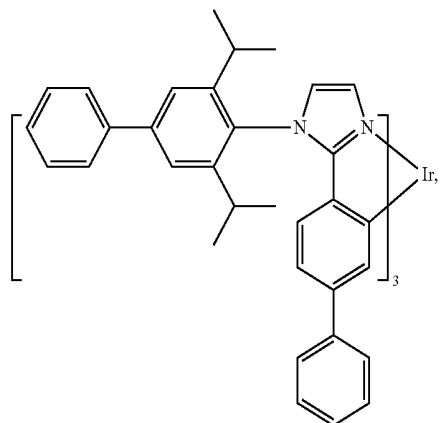
Compound 25
