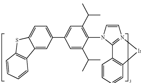
Compound 32
