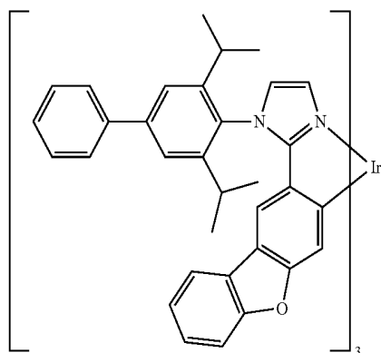
Compound 7
