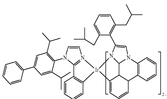
Compound 69
