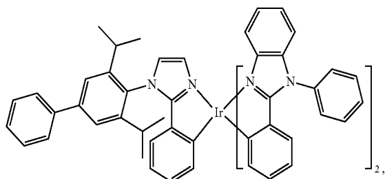
Compound 64
