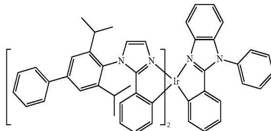
Compound 53
