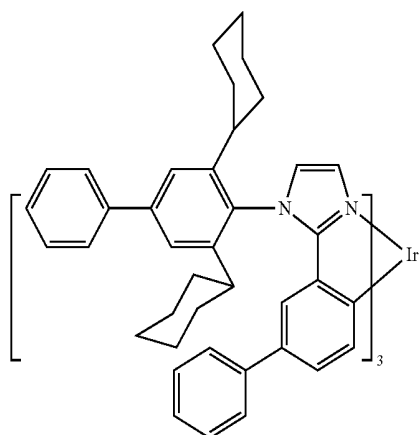
Compound 14
