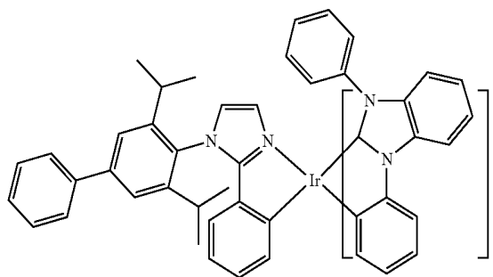
Compound 67
