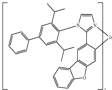
Compound 7
