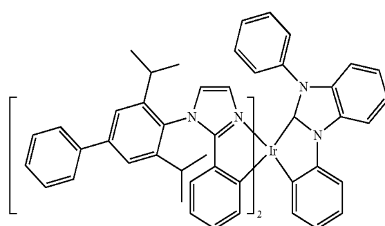
Compound 56
