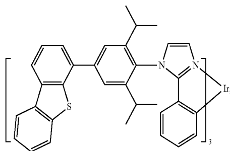
Compound 33
