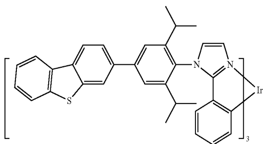
Compound 33
