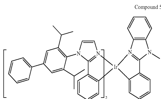
Compound 52
