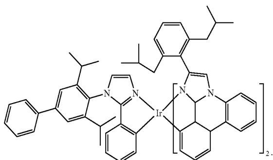
Compound 69
