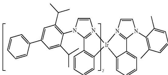
Compound 50
