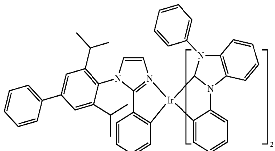
Compound 68
