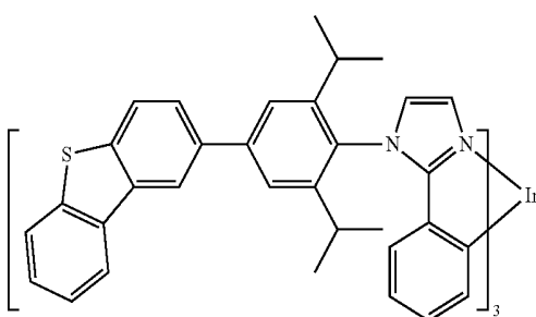
Compound 32
