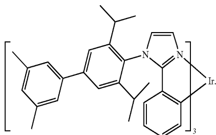
Compound 66
