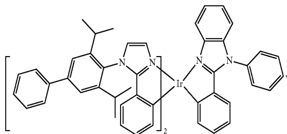
Compound 53
