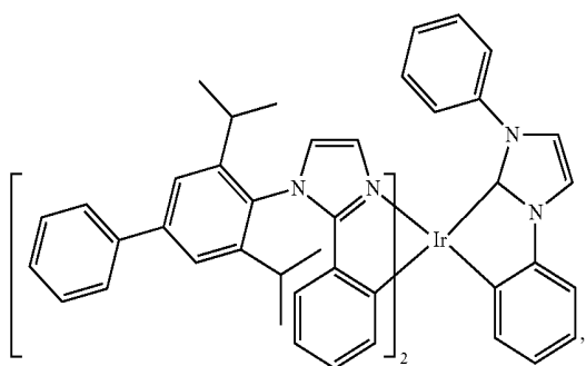
Compound 55
