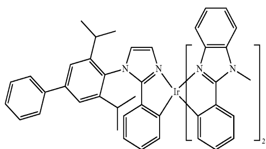
Compound 63
