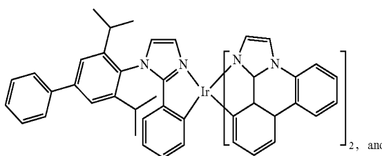
Compound 69
