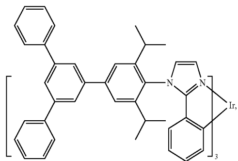
Compound 31
