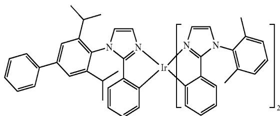
Compound 61
