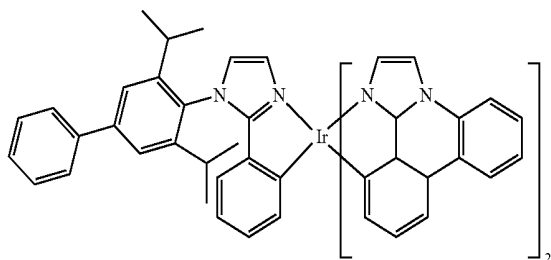
Compound 68
