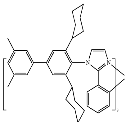
Compound 9
