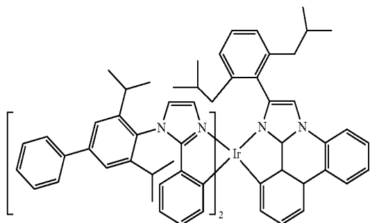
Compound 59
