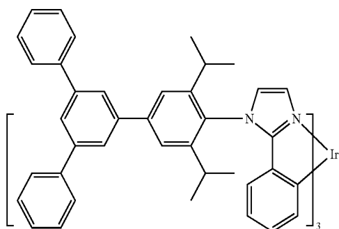
Compound 32
