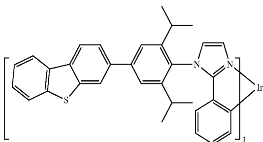
Compound 33
