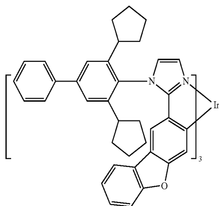
Compound 18
