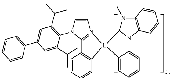
Compound 66
