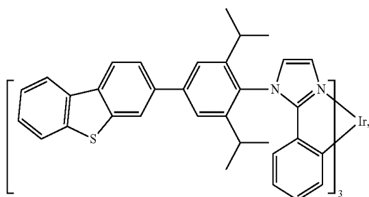
Compound 33
