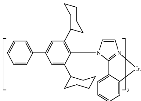
Compound 3
