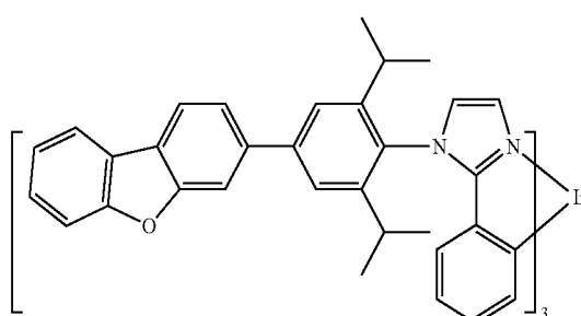
Compound 36
